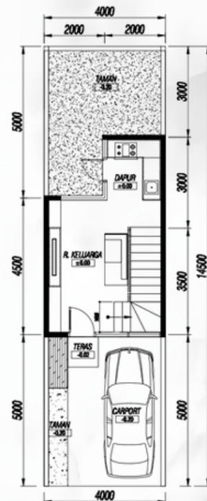
DENAH LT. 1 S 1: 100
