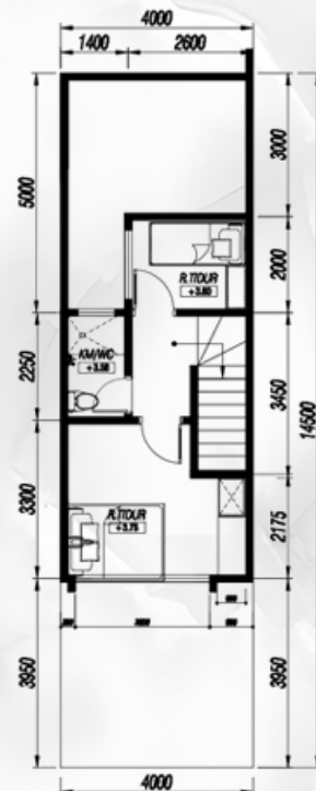
DENAH LT. 2 S 1: 100
