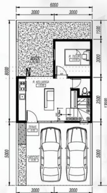
HIMAWARI DENAH LT. 1 6 X 13
